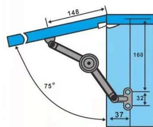
75° Installation
