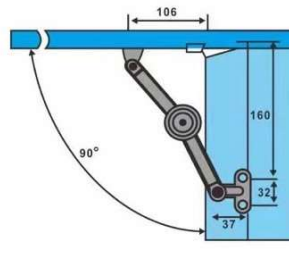
90° Installation
