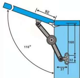
110° Installation
